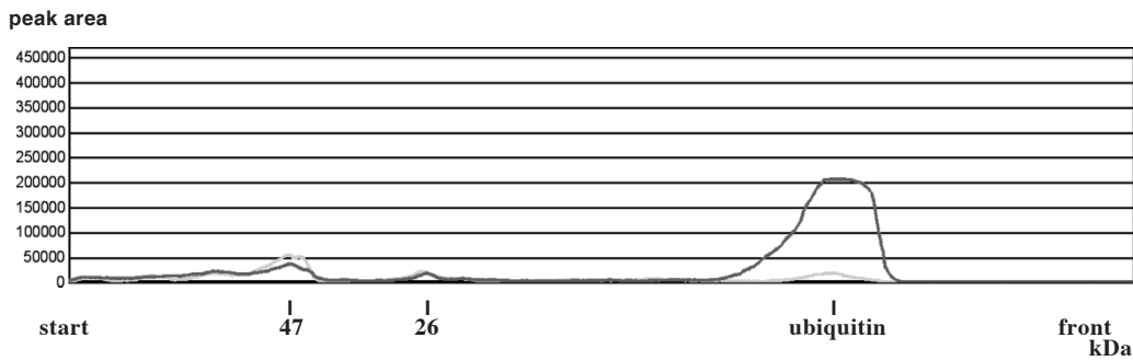
Fig. 7b. Overlay of the densitogram curves before and after ubiquitylprotein-isopeptidase incubation of the heart muscle APFII. Fig. 7b shows the densitogram curves before (green lane) and after (red lane) enzyme incubation of 200 µg heart muscle-APFII and 25 µg ubiquitylprotein-isopeptidase (see material). The batches incubated with ubiquitylprotein-isopeptidase had a final concentration of 50 mM Tris/HCl, 1 mM DTE, 50 µM PMSF and 5 µg/ml leupeptine, pH 8.0. After incubation at 37 °C for a given time (60 min) in a waterbath the reaction was irreversible inhibited by a final concentration of 5mM M iodacetamide and 10 % w/v TCA (final concentration 5 % TCA, 20 min, 0 °C). Each batch was incubated with 25 µg ubiquitylprotein-isopeptidase. Both densitograms were overlaid to estimate the release of unconjugated (free) ubiquitin.
