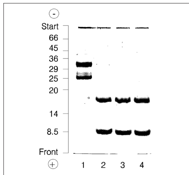
Fig.1. Reaction products of isopeptidase activity. Reaction mixtures for isopeptidase activity contained in a final volume of 50 µl 50 mM Tris/HCl, 1 mM DTE, 5 mM MgCl 2 , 1 mM ATP, 1 mM EGTA, 0.2 mg/ml first order and second order ubiquityl-calmodulin conjugates and the indicated amounts of affinity-purified isopeptidase activity. Incubation was stopped after 60 min by adding 60 µl of Laemmli sample buffer containing 10 mM EGTA and heating to 96 ° C for 5 min. The reaction mixtures were analyzed on a 12.5 % Weber-Osborne gel.
