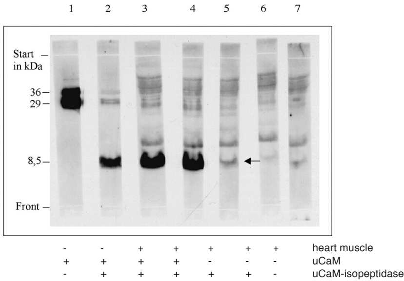
Fig. 6a. Cleavage of Ubiquitin-conjugates in the heart muscle with ubiquitylprotein-isopeptidase.
