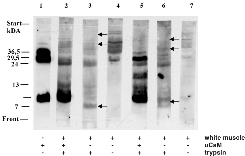
Fig. 10a. Trypsin-incubation of white muscle extract and APFII. Fig. 10a shows the cleavage of internal and external ubiquitin-conjugates of the white muscle with trypsin. The incubation batches have a final concentration of 5 µg/ml leupeptine. The batches were incubated for 30 min in 37 °C in a waterbath. The reaction was stopped by adding trichloroacetic acid (final concentration 5 % w/v TCA, 20 min 0 °C). After centrifugation for 5 min in an Eppendorf centrifuge 5415 (Eppendorf, Hamburg) at 16000 x g the pellet were solved in the sample buffer for Laemmli system and then blotted on PVDF-membrane (see materials). Lane 1: 8.5 µg ubiquityl-calmodulin conjugates and 2 µg unconjugated ubiquitin Lane 2: 200 µg white muscle extract, 8.5 µg ubiquityl-calmodulin conjugates and 65 µg trypsin Lane 3: 200 µg white muscle extract and 65 µg trypsin Lane 4: 200 µg white muscle extract Lane 5: 200 µg white muscle APFII, 8.5 µg ubiquityl-calmodulin conjugates and 65 µg trypsin Lane 6: 200 µg white muscle APFII and 65 µg trypsin Lane 7: 200 µg white muscle APFII
