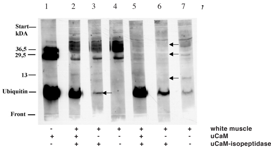
Fig. 8a. Cleavage of Ubiquitin-conjugates in the white muscle with ubiquitylprotein-Isopeptidase. Fig.8a shows the cleavage of ubiquitin-conjugates of the extract and APFII after anion-exchange chromatography from the white muscle (batch 2-7). The incubation batches contained with a final concentration of 5 µg/ml leupeptine and depending on batch 5 mM iodacetamide. All batches were incubated for 60 min in 37 °C in a waterbath. The reaction was stopped by adding trichloroacetic acid (final concentration 5 % w/v TCA, 20 min 0 °C).
