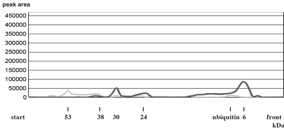
Fig. 9c. Overlay of the densitogram curves before and after trypsin-incubation of the heart muscle APFII Fig. 9c shows the enzyme incubation of 200 µg heart muscle-APFII with 65 µg trypsin (see Material). The batches, incubated with trypsin had a final concentration of 20 mM Tris/HCl, 20 mM \beta -mercaptoethanol, pH 8.0. After incubation at 37 °C for a given time (30 min) in a waterbath, the reaction were irreversible inhibited by an final concentration of 10 % w/v TCA (final concentration 5 % TCA, 20 min, 0 °C).
